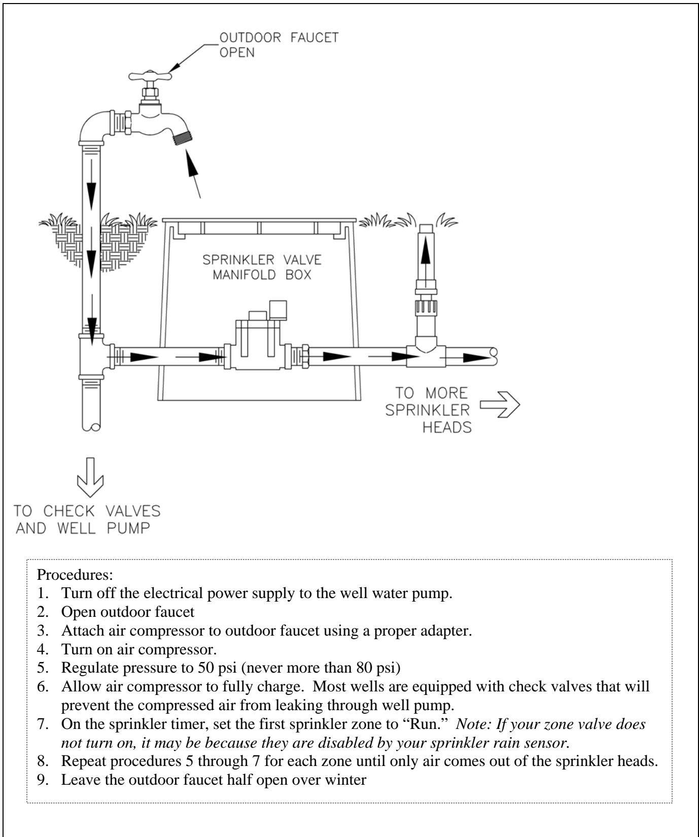
Figure 3. Winterizing Sprinkler System Connected to Well
