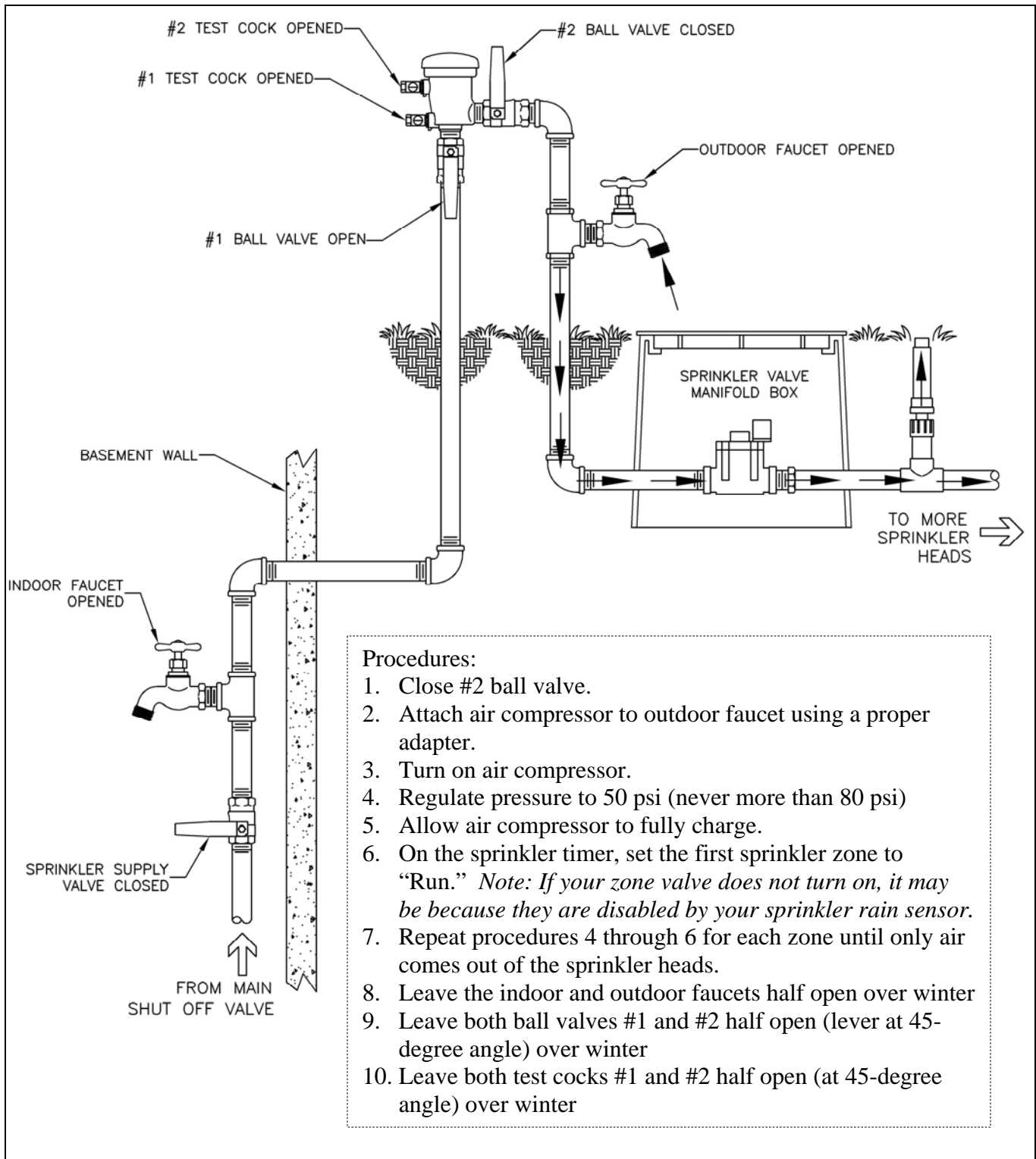
Figure 1B. Winterizing Sprinkler System Using Air Compressor
