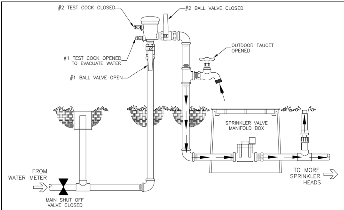
Figure 2B. Winterizing Sprinkler System Using Air Compressor
