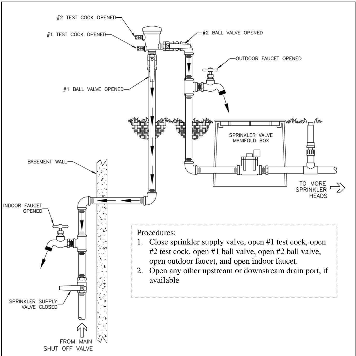
Figure 1A. Winterizing Pressure Vacuum Breaker Assembly Using Gravity
