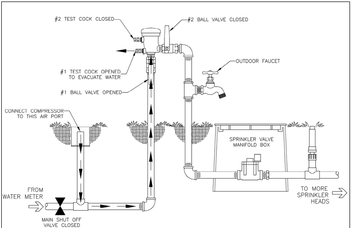
Figure 2A. Winterizing Pressure Vacuum Breaker Assembly Using Air Compressor
